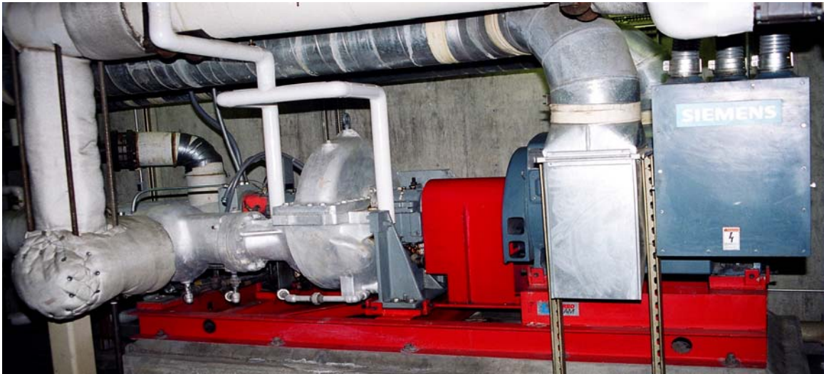
Photo of steam turbine and generator
