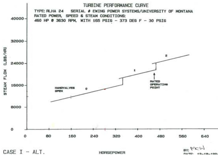
TURBINE PERFORMANCE CURVE WITH HAND VALVES
